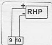
RHP POLA sensor probe connection
