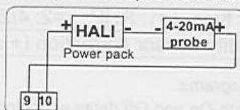
4-20mA sensor probe connection
